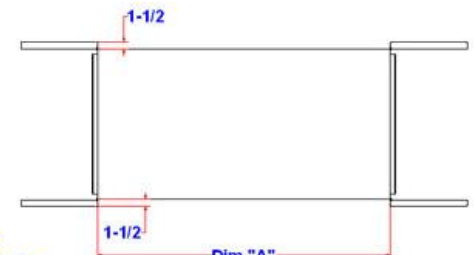
Top view with doors open showing hinge offset requirements
